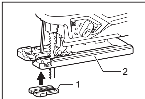
► 1. Anti-splintering device 2. Tool base
