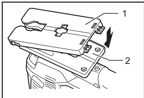
► 1. Cover plate 2. Tool base
